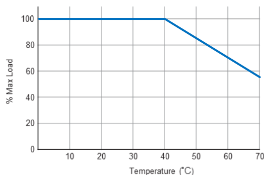
OUTPUT POWER DERATING CURVE
